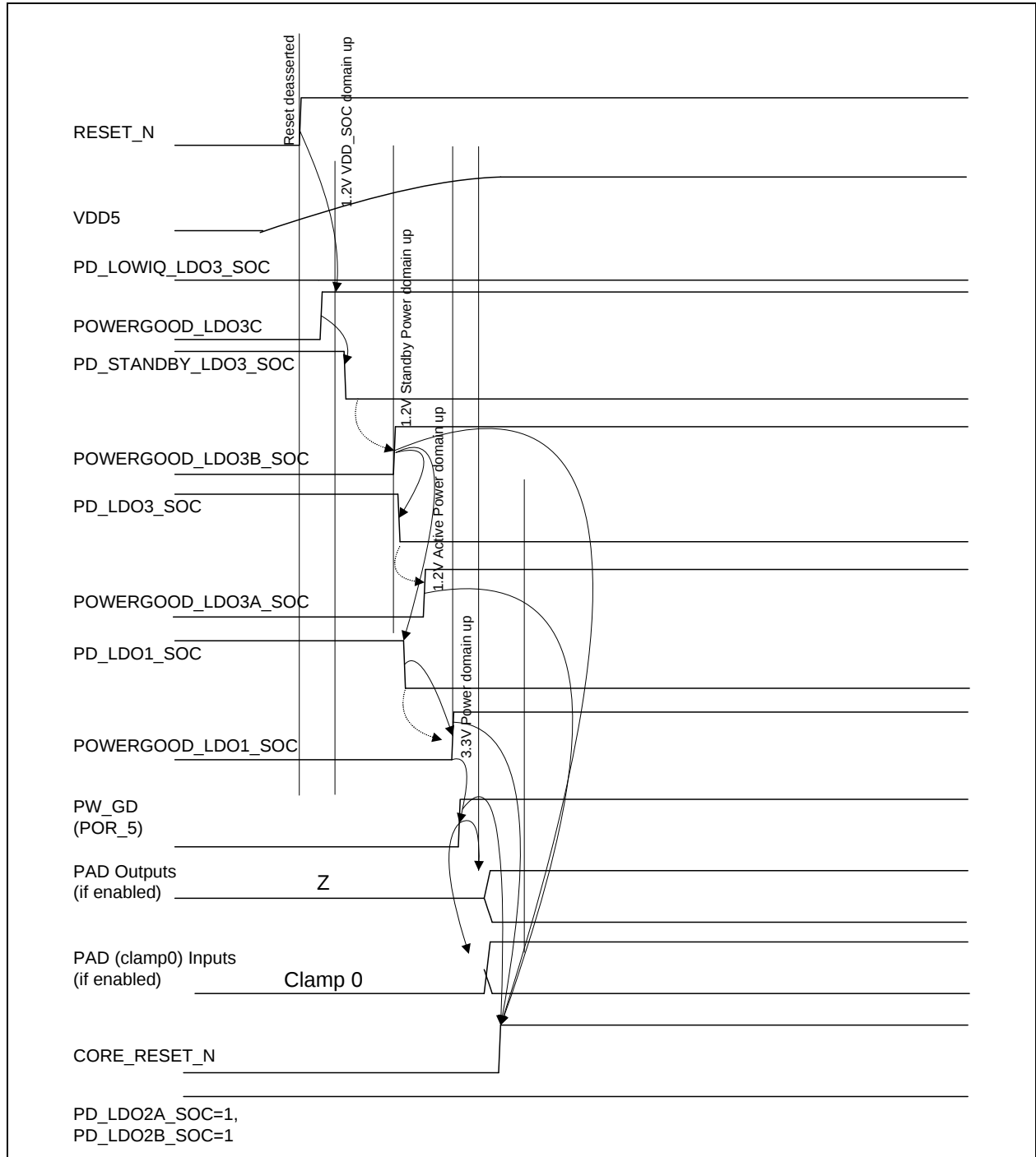
FIGURE 15-6: POWER-ON SEQUENCING
