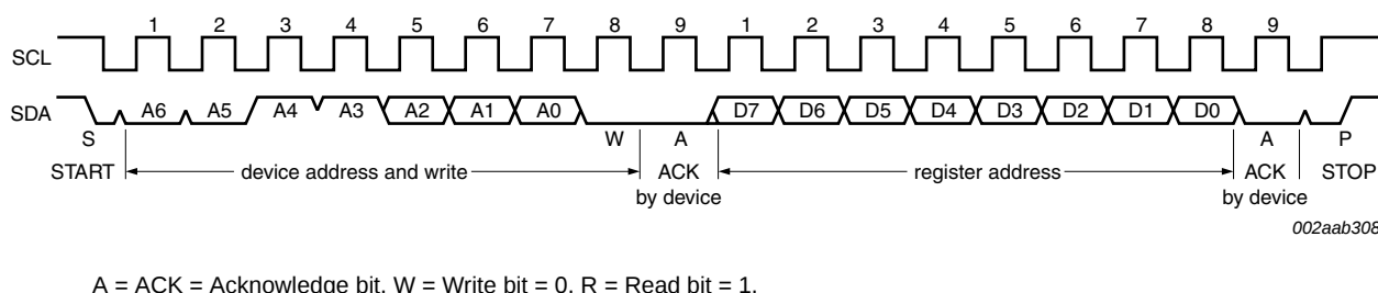
Fig 8. SMBus/I 2 C-bus write to the Pointer register
