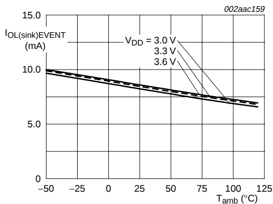
Fig 16. \overline{EVENT} sink current at 0.4 V versus temperature
