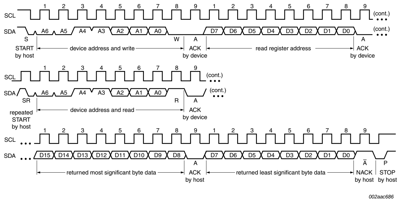
Fig 12. SMBus/I²C-bus write to Pointer register followed by a repeated START and an immediate data word read
