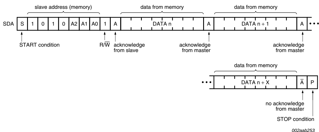
Fig 21. Sequential read timing
