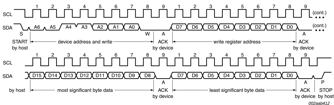
Fig 11. SMBus/I²C-bus write to the Pointer register followed by a write data word
