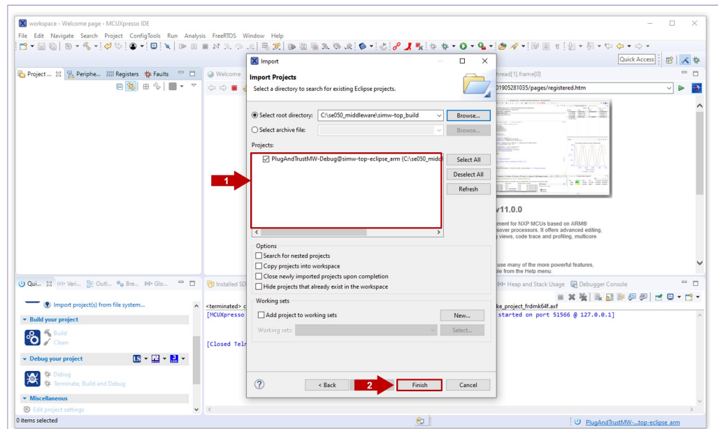
Figure 28. Import EdgeLock SE050 Plug & Trust middleware
