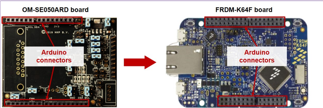
Figure 7. Arduino connectors of OM-SE050ARD and FRDM-K64F boards
