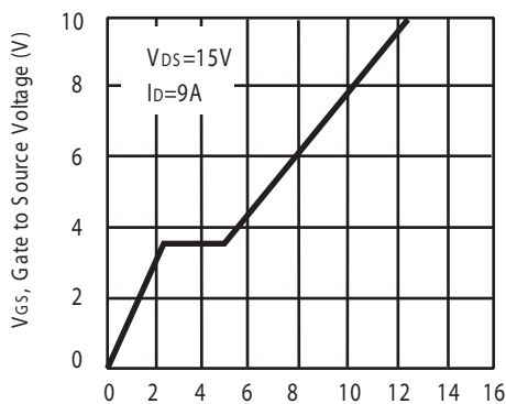
Figure 9. Gate Charge
