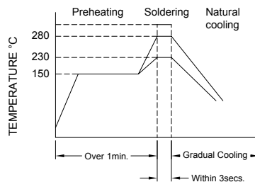
Figure 3. Hand Soldering
