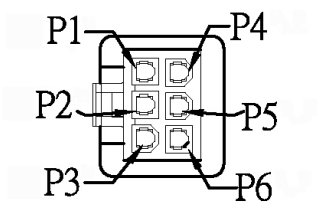
Output cable plug pin assignment
