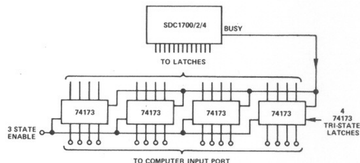
Suggested External Computer Interface Circuitry
