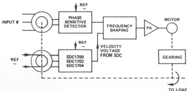
Diagram showing the velocity voltage being used to stabilize a closed loop control system.
