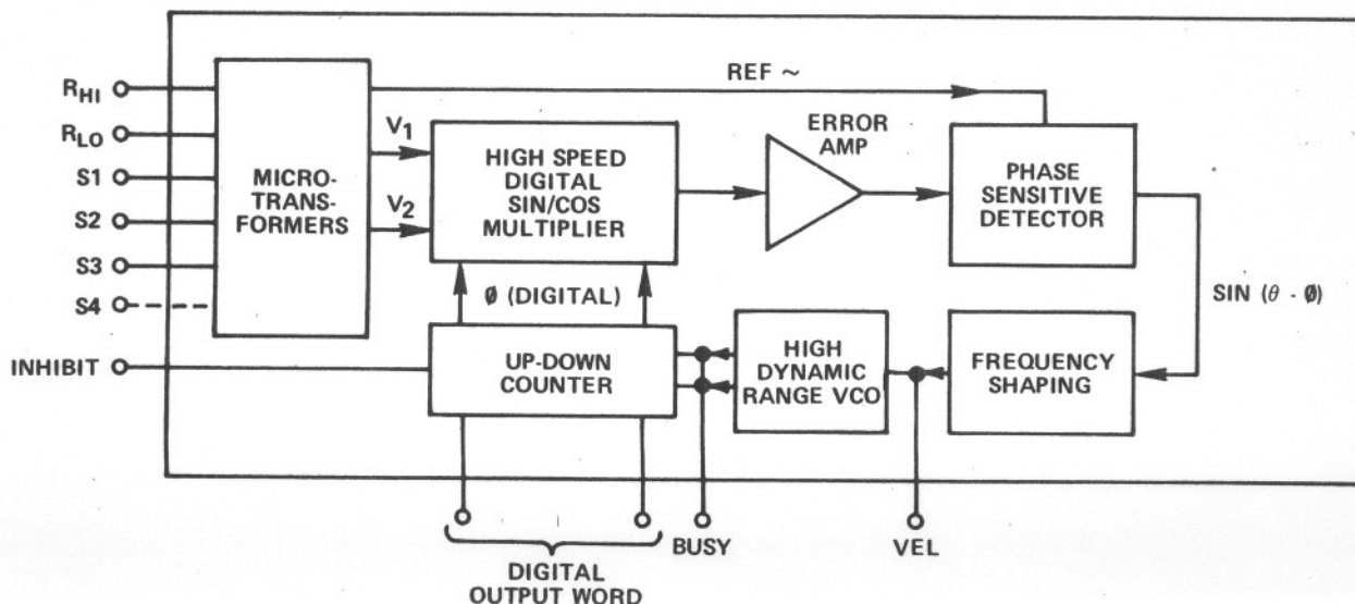
Functional Diagram of the SDC1700/2/4
