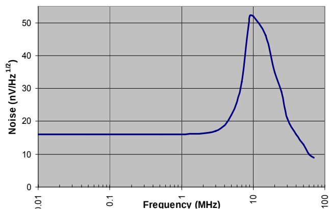
Dark Output Noise @ Gain 300
