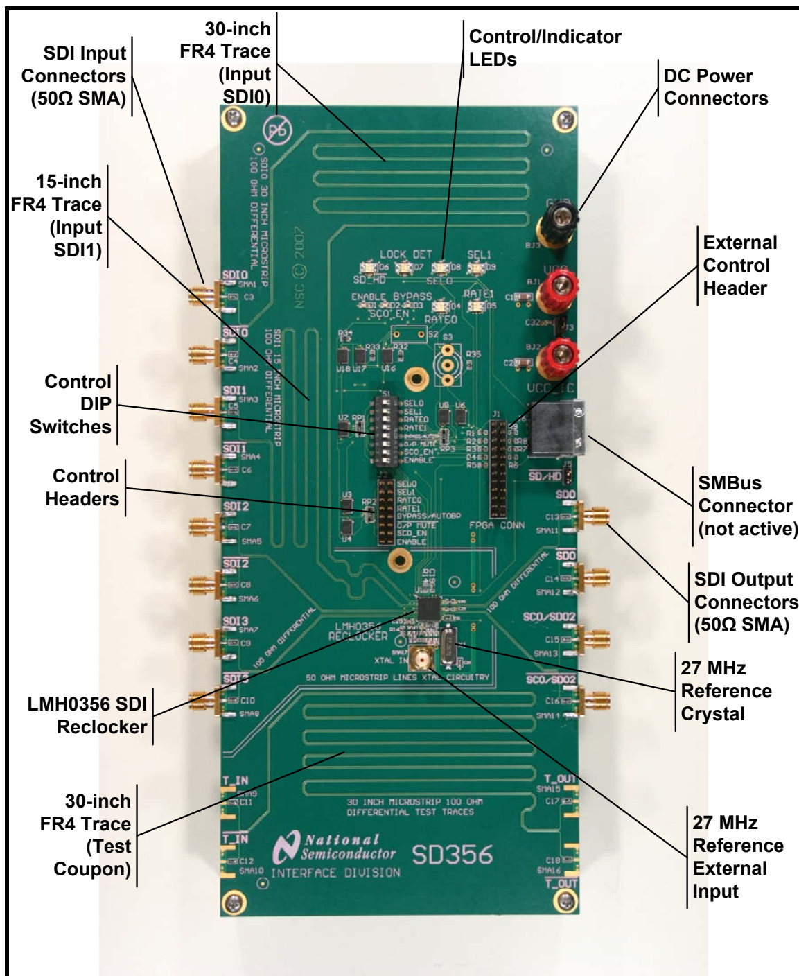
Figure 1. SD356EVK board
