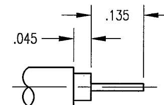
CABLE TRIMMING DIMENSIONS
