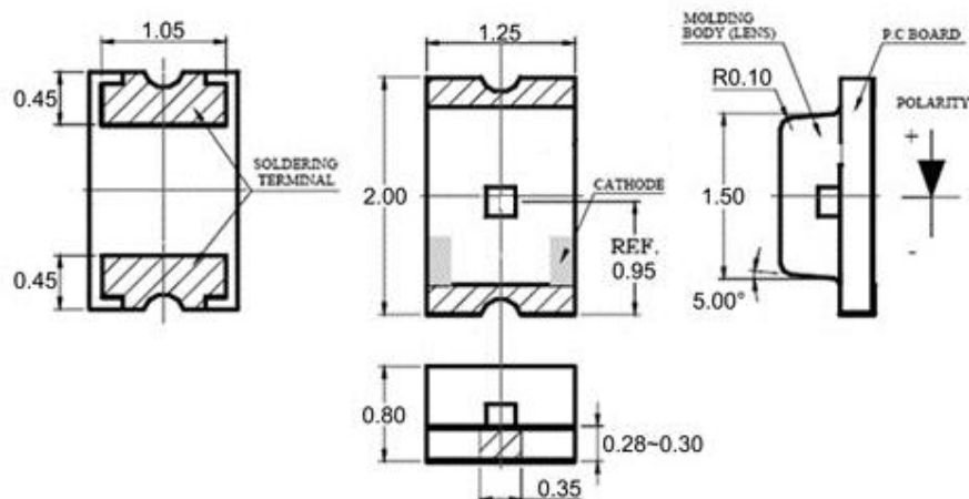
0805 PACKAGE DIMENSIONS, MM
