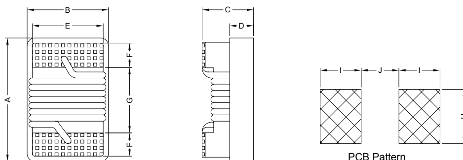
PCB Pattern
