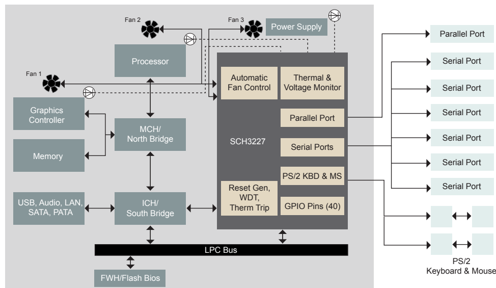
System Controller Hub Application Diagram
