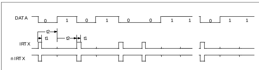
FIGURE 10-13: IRDA TRANSMIT TIMING
