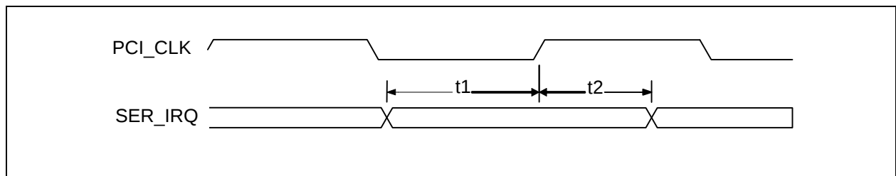
FIGURE 10-15: SETUP AND HOLD TIME
