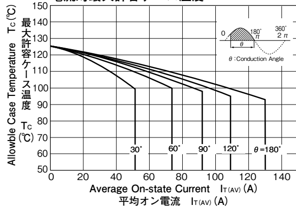
Output Current (B2; Two pulse bridge connection)
