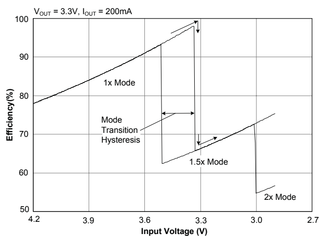
Efficiency — 200mA
