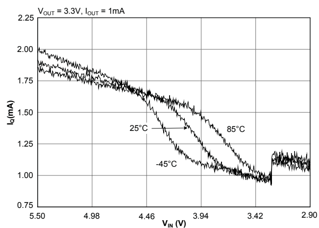
Quiescent Current
