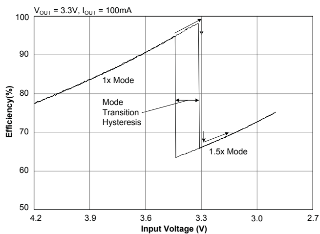
Efficiency — 100mA
