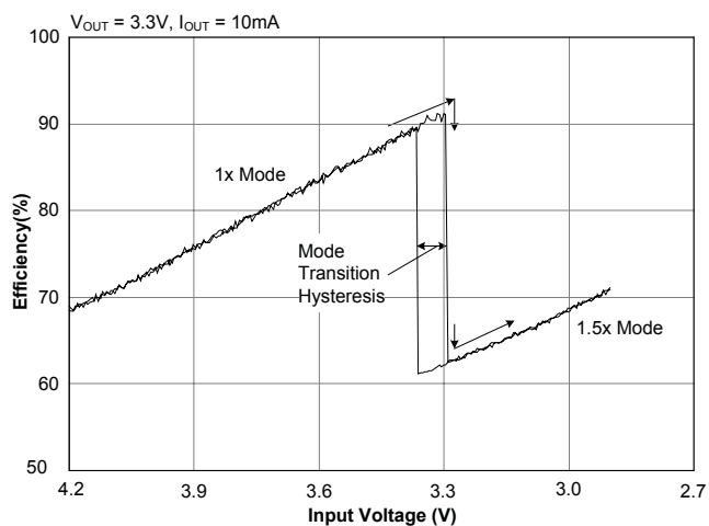
Efficiency — 10mA
