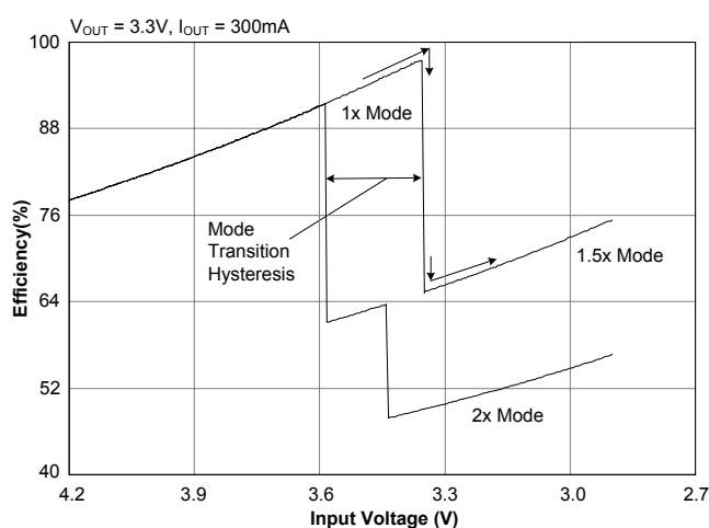
Efficiency — 300mA
