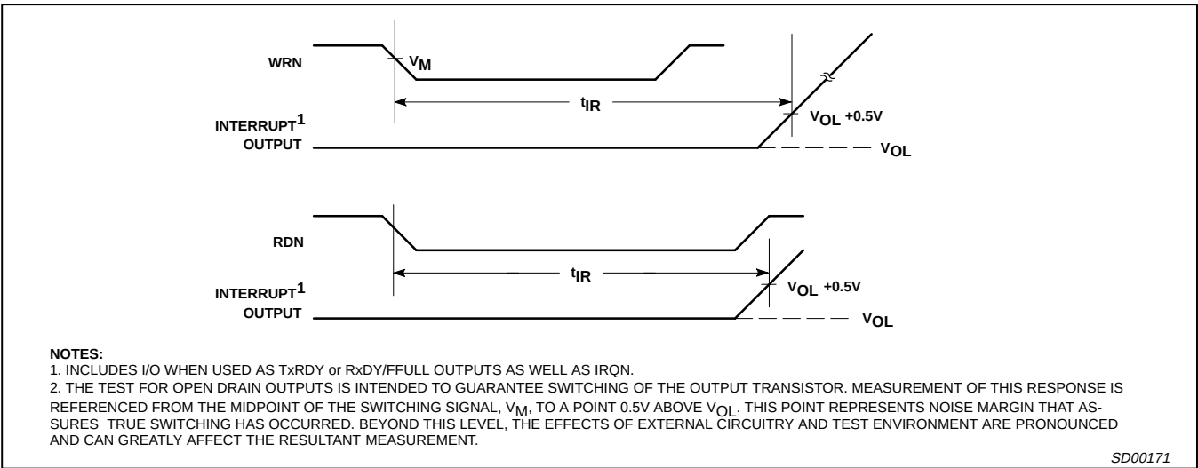
Figure 9. Interrupt Timing
