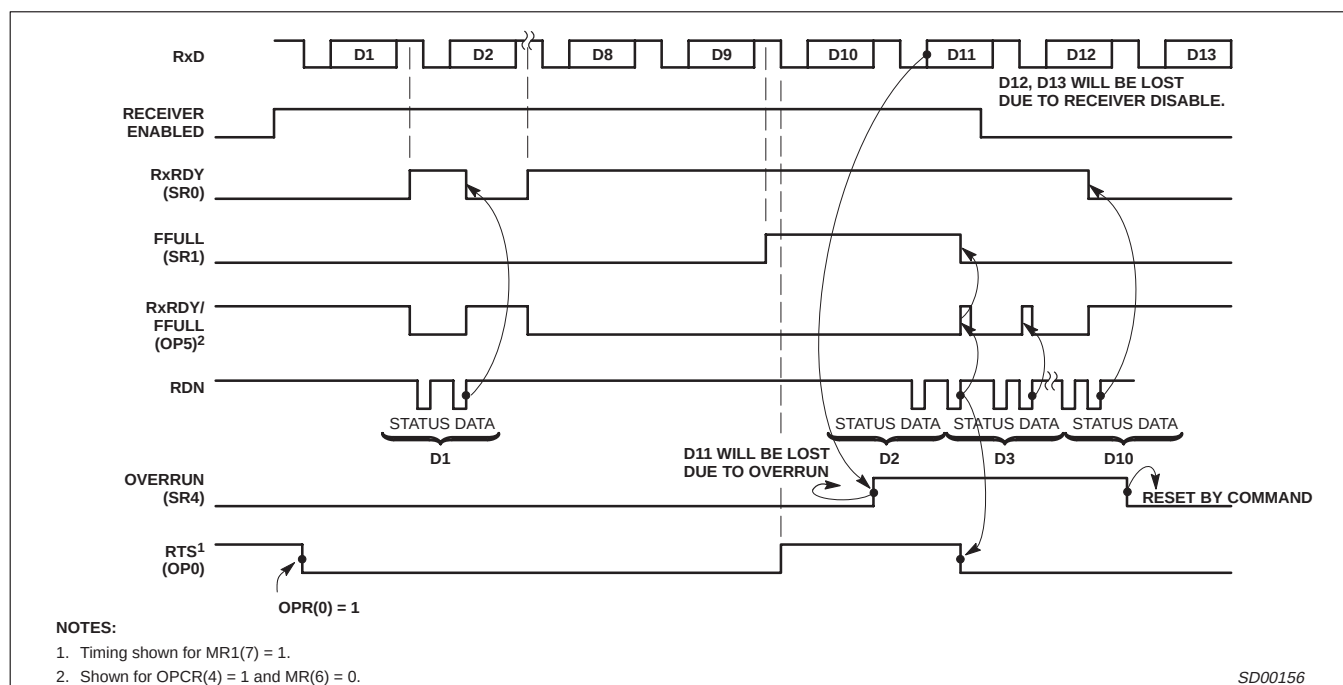
Figure 11. Receiver Timing
