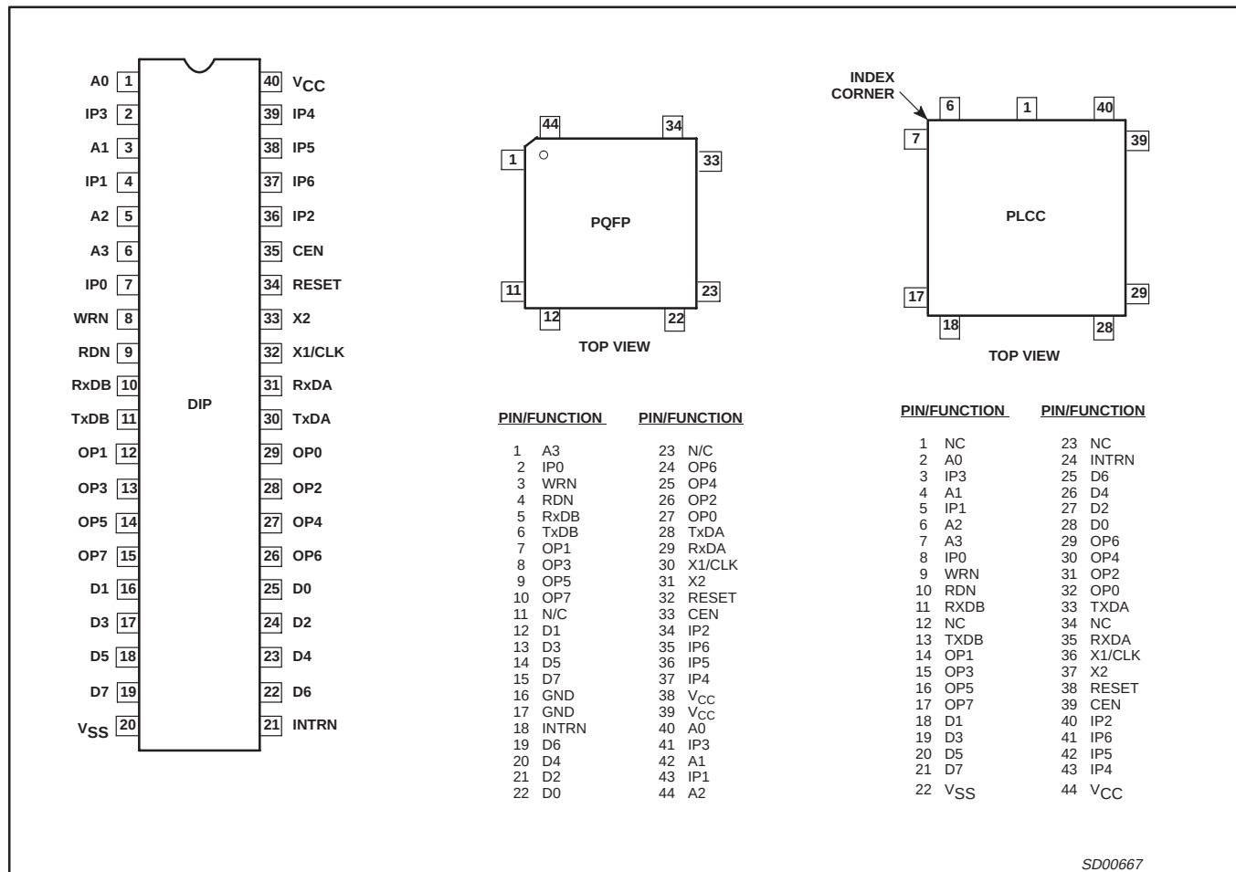
Figure 1. Pin Configurations
