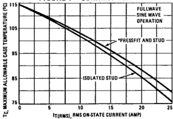
FIGURE 1 – CURRENT DERATING
