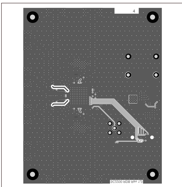
SC2200 EV Kit—Bottom Layer 4
