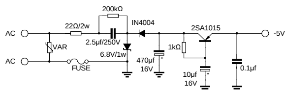
Supply Circuit
