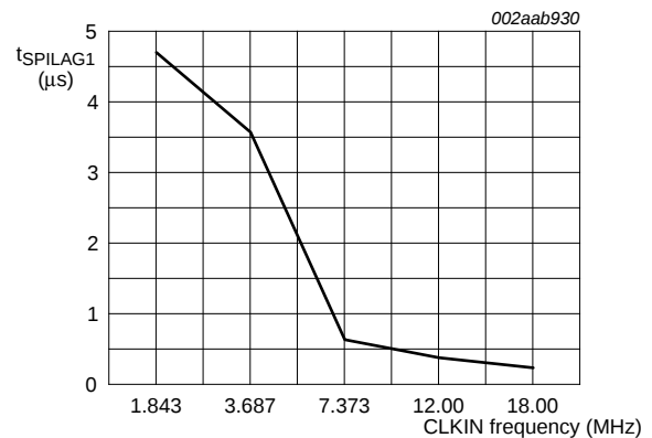
Fig 22. t_{\text{SPILAG1}} as a function of CLKIN frequency
