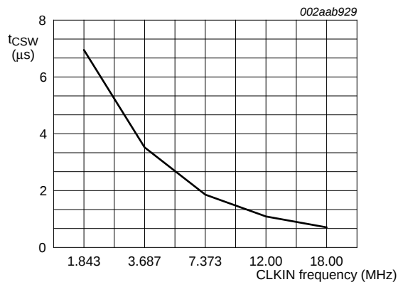
Fig 21. t_{\text{CSW}} as a function of CLKIN frequency
