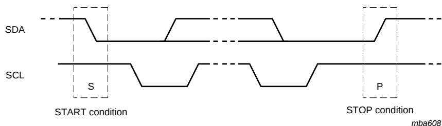
Fig 13. START and STOP conditions
