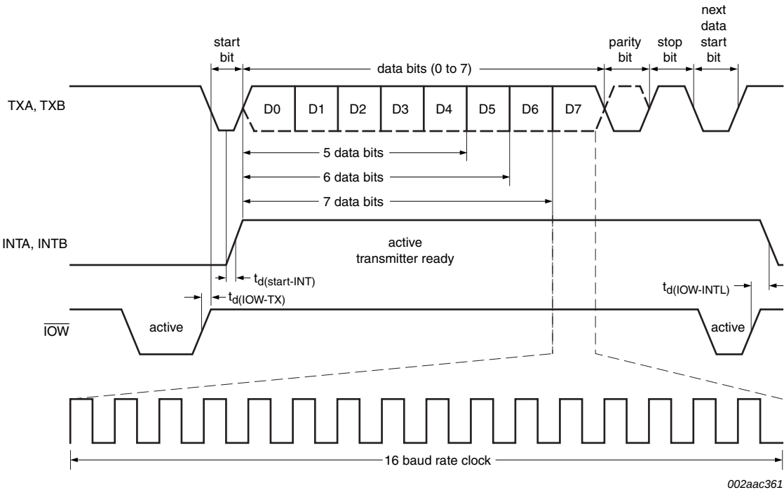
Fig 17. Transmit timing
