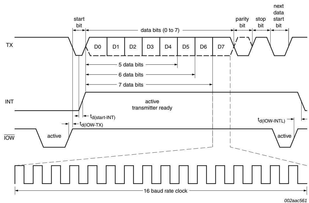
Fig 12. Transmit timing
