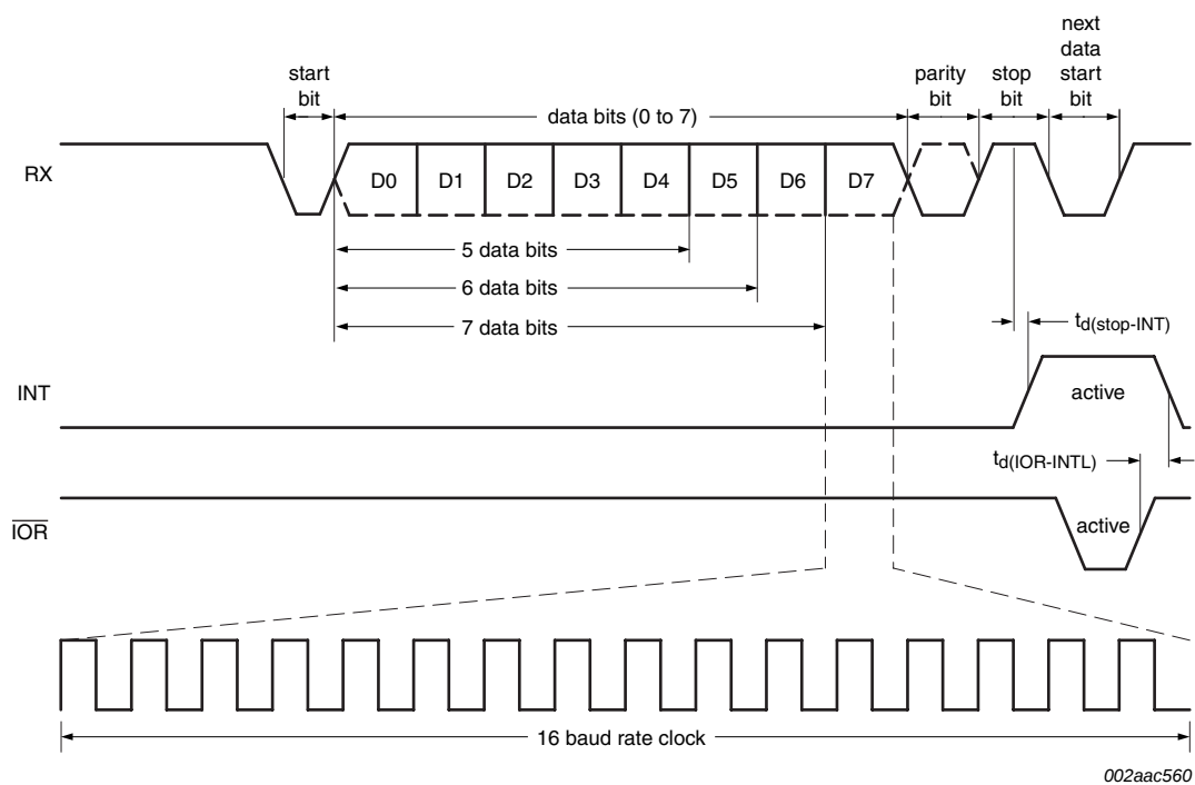
Fig 11. Receive timing
