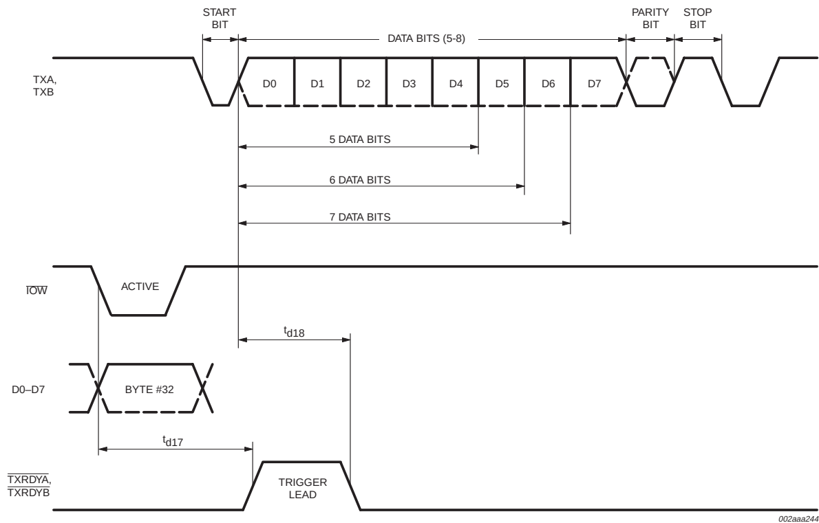
Fig 22. Transmit ready timing in FIFO mode.
