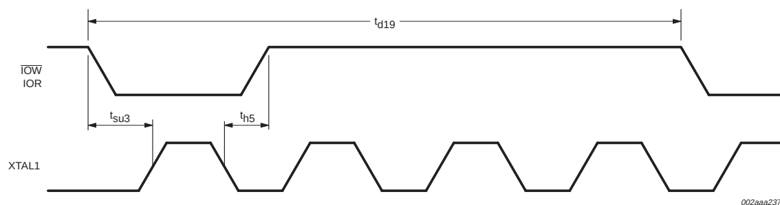
Fig 15. Alternate read/write strobe timing.
