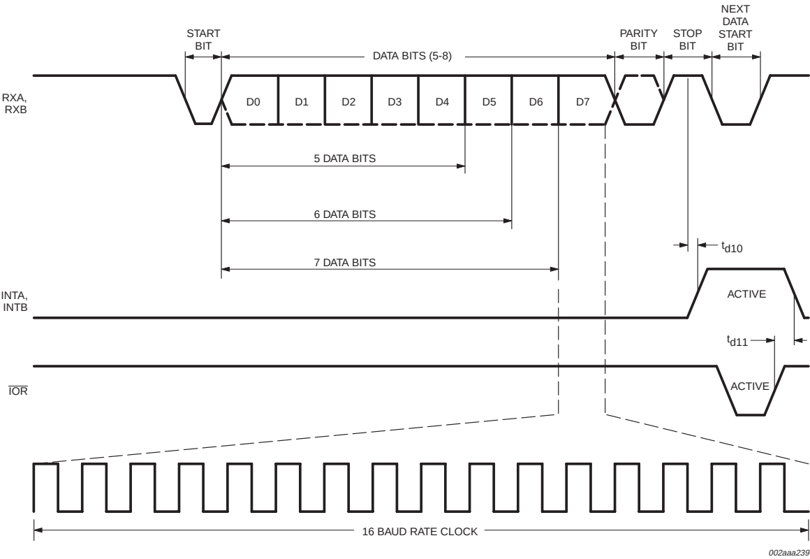
Fig 17. Receive timing.
