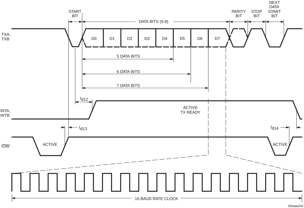
Fig 20. Transmit timing.
