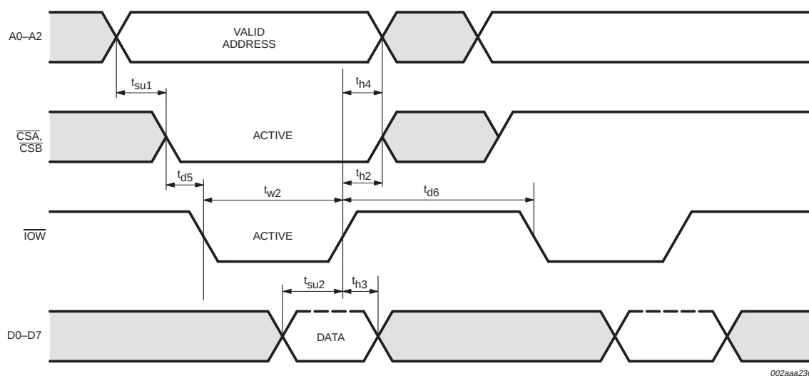
Fig 14. General write timing.
