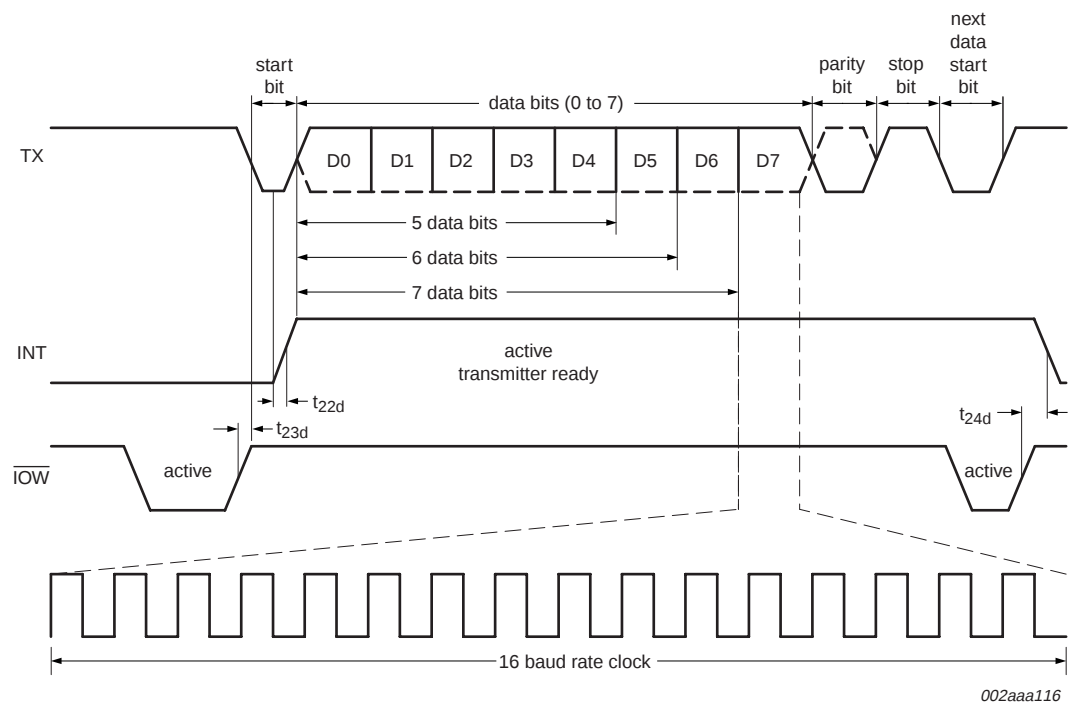
Fig 10. Transmit timing
