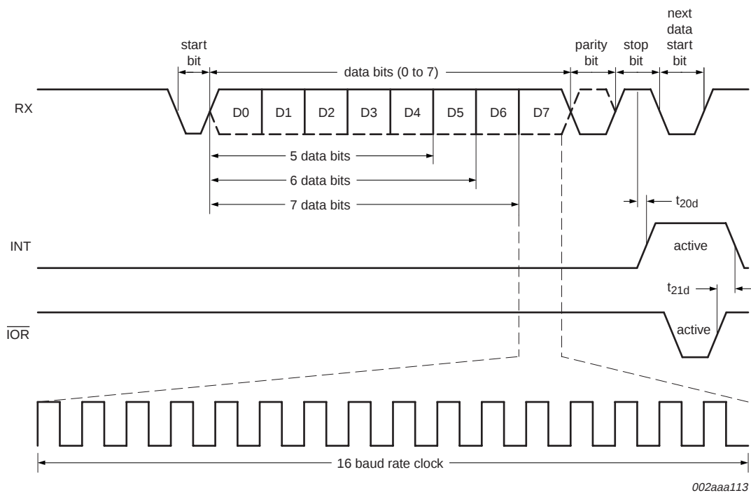
Fig 9. Receive timing
