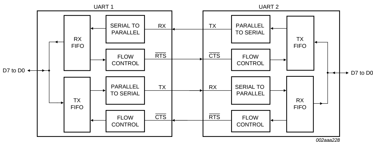
Fig 6. Autoflow control (auto-RTS and auto-CTS) example
