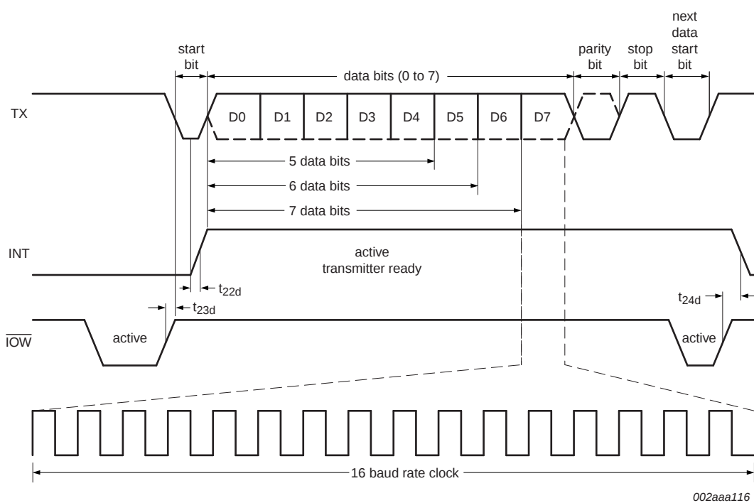
Fig 21. Transmit timing
