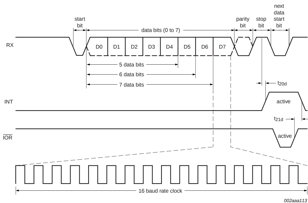
Fig 18. Receive timing
