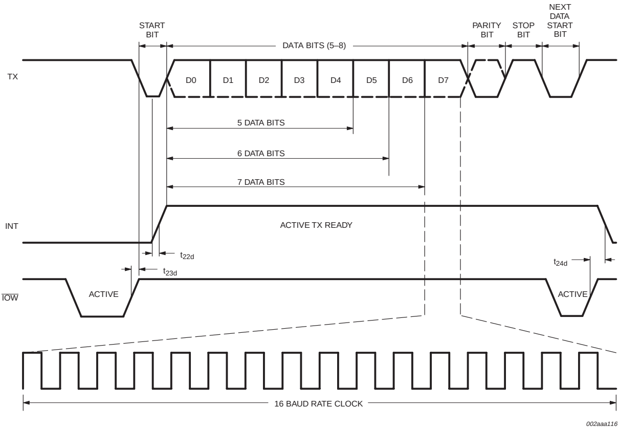
Fig 14. Transmit timing.
