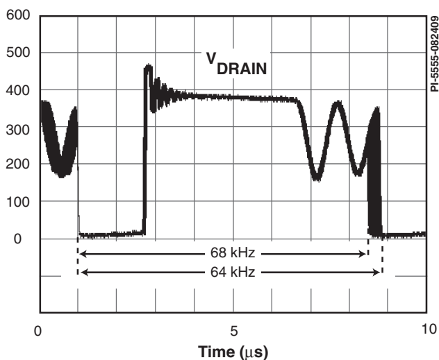
Figure 4. Frequency Jitter.
