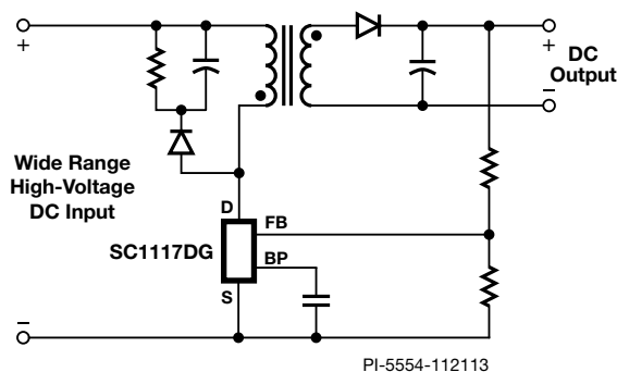
Figure 1. Typical Application Schematic, Flyback Non-Isolated.
