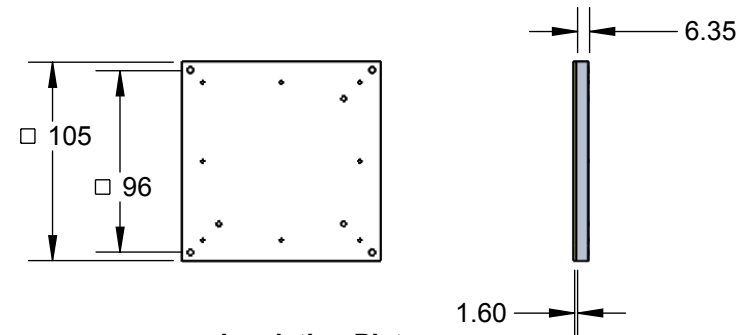
Insulation Plate Scale 1:4
