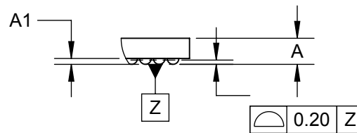
DETAIL A SCALE 4 : 1
