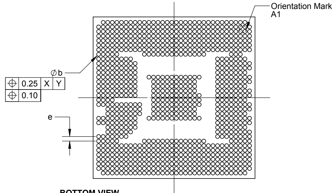
BOTTOM VIEW
