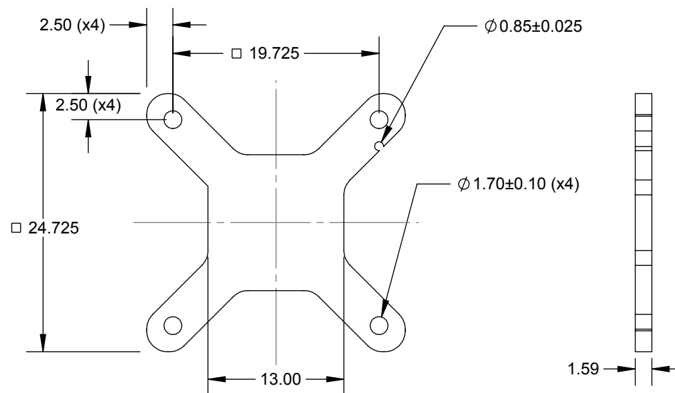
Insulating Plate Detail
