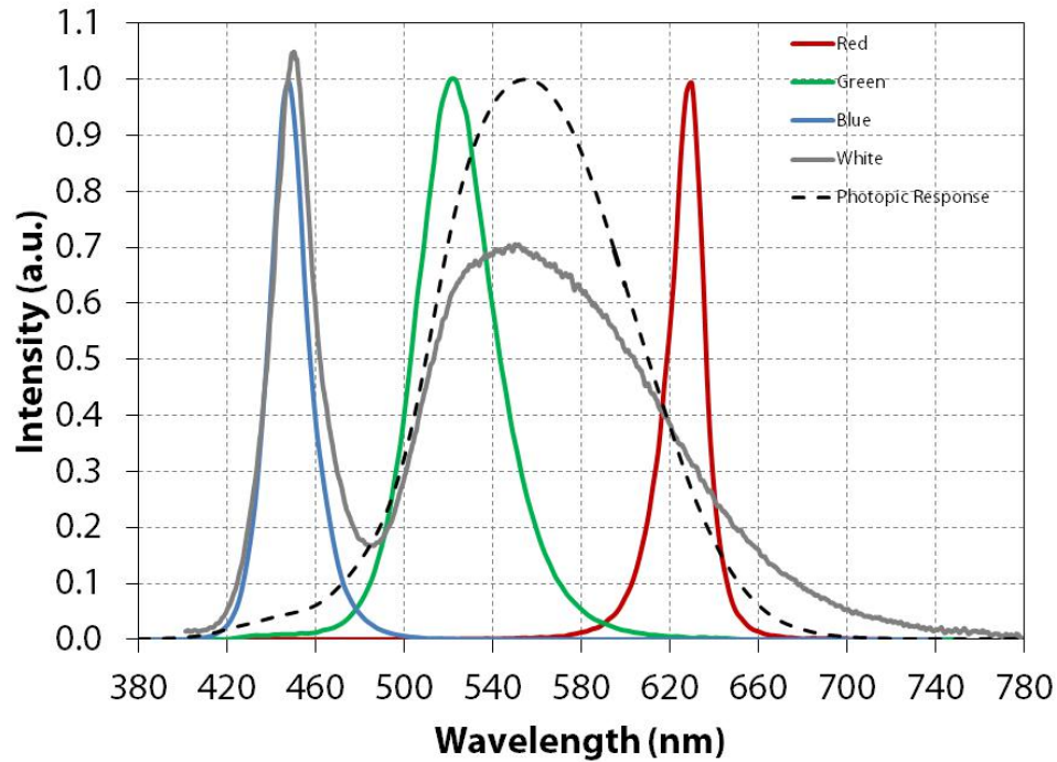
SBM-40-LC -RGBW Spectrum 8
