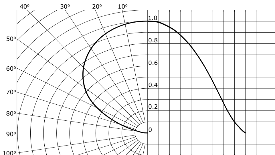
SBM-40-LC -RGBW Angular Distribution
