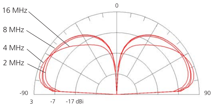
SB-V35 above 8-18 Ground Radials
