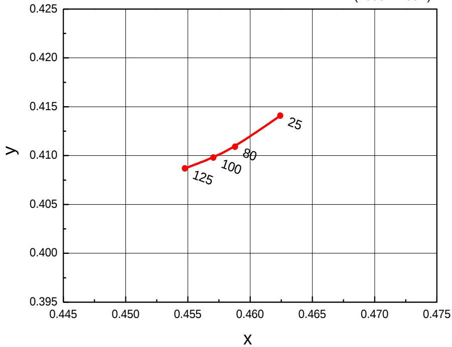
Fig 8. Chromaticity Coordinate vs. Junction Temperature, I_F=50\text{mA}
