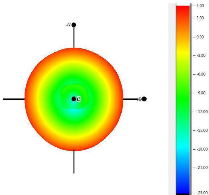
3D Radiation Pattern (Unit: dBi)
