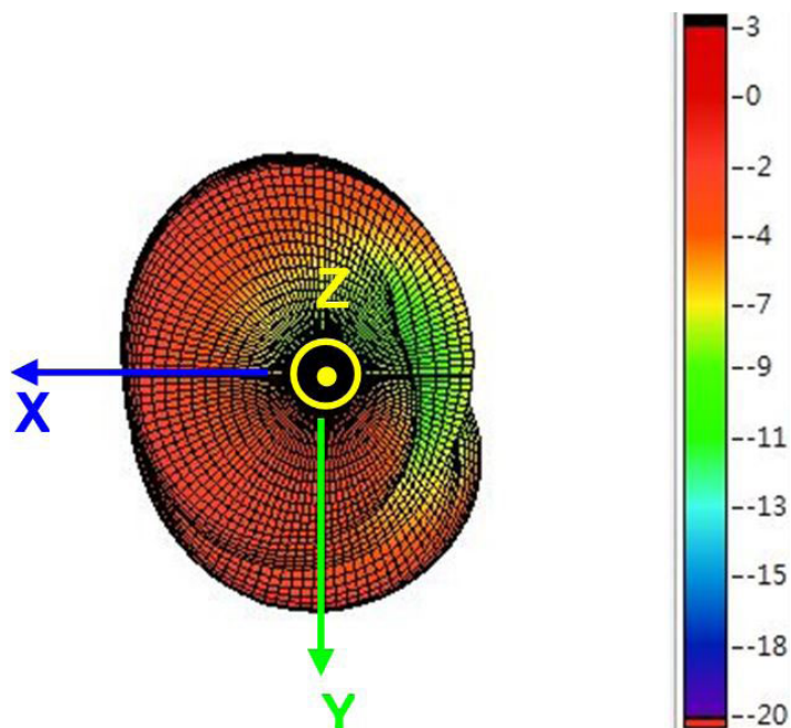
Radiation Pattern 2442MHz
