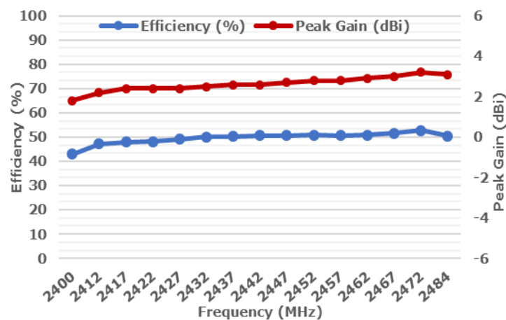
Efficiency V's Frequency 2442MHz
