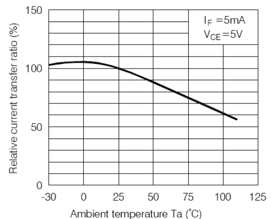
Figure 6: Relative CTR (%) vs. Temperature ( ^\circ\text{C} )
