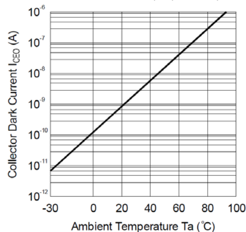
Figure 8: Collector Dark Current ( I_{CEO} ) vs. Temperature ( ^\circ\text{C} )
