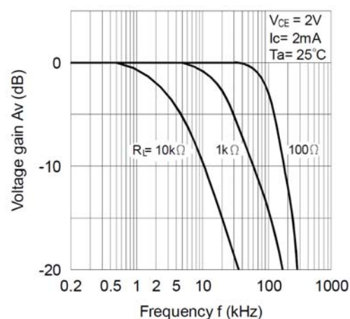
Figure 10: Frequency Response Characteristics
