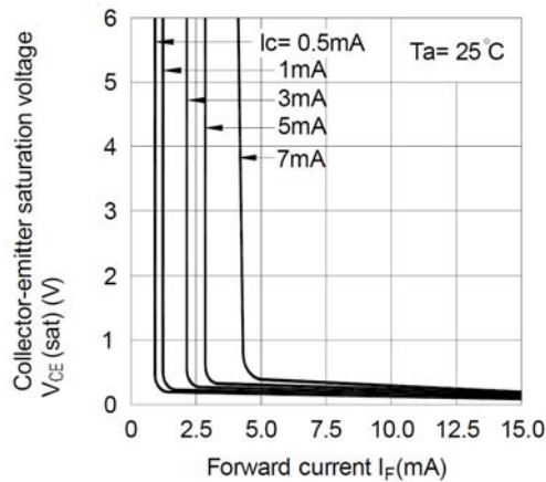
Figure 3: Collector-Emitter Saturation Voltage ( V_{CE(SAT)} ) vs. Forward Current ( I_F )
