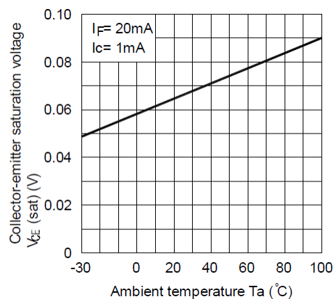
Figure 7: Collector-Emitter Saturation Voltage ( V_{CE(SAT)} ) vs. Temperature ( ^\circ\text{C} )
