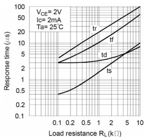
Figure 9: Response Times vs. Load Resistance ( R_L )
