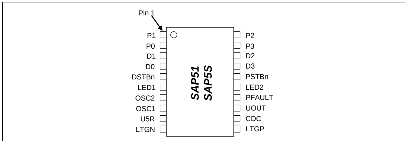
Figure 7.1 SAP51/SAP5S SOP20 Package Pin Assignment
