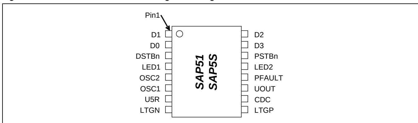
Figure 7.2 SAP51 / SAP5S SOP16 Package Pin Assignment
