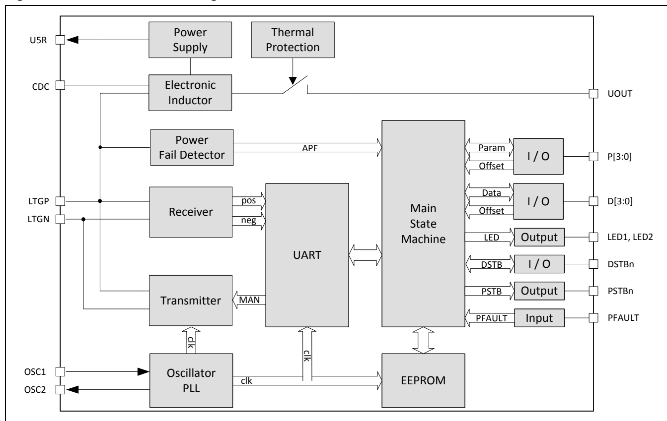
Figure 3.1 Functional Block Diagram
