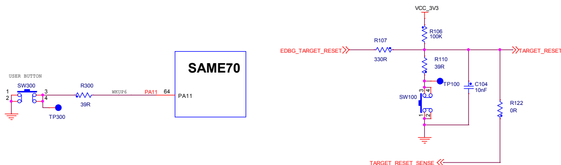
Figure 4-20 Mechanical Button Schematic
