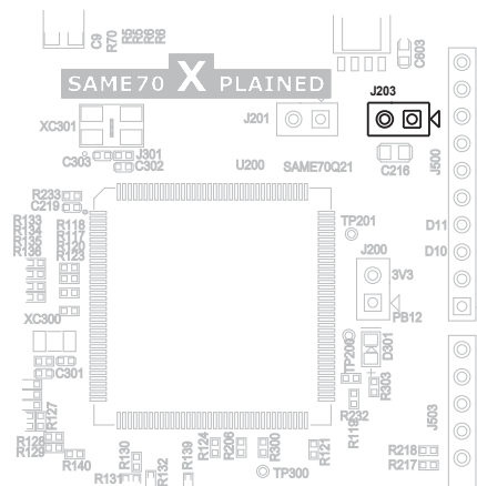
Figure 4-14 VCC_MCU_P3V3 Connector Placement J203
