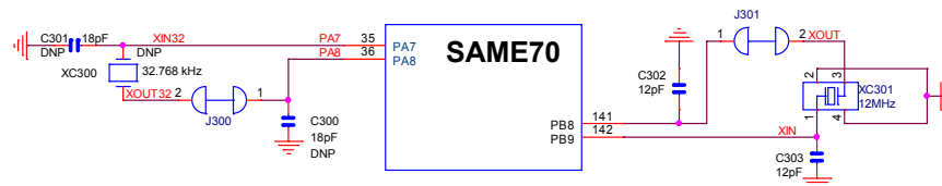
Figure 4-19 SAM E70 Crystals Schematic
