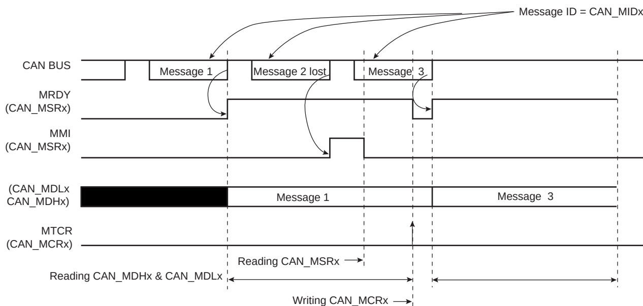
Figure 40-11. Receive Mailbox
