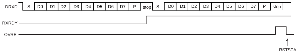
Figure 23-7. Receiver Overrun
