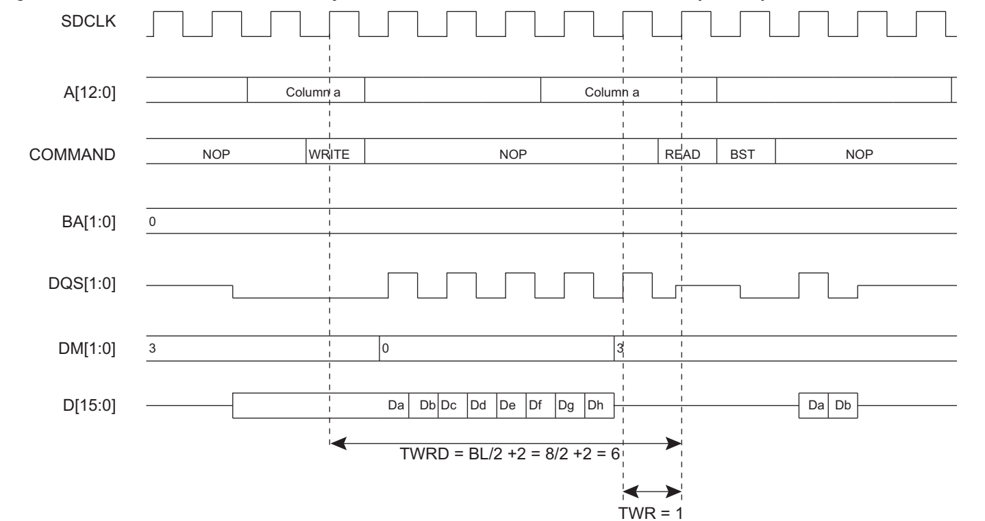
Figure 29-8. Write Command Followed By a Read Command Without Burst Write Interrupt, Low-power DDR1-SDRAM Device
