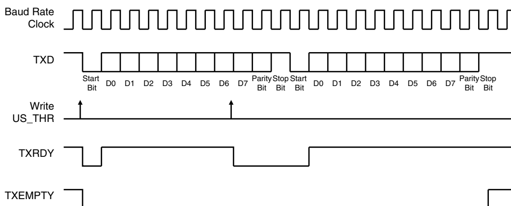
Figure 32-7. Transmitter Status
