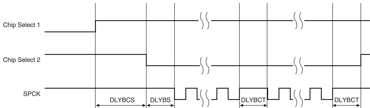
Figure 30-9. Programmable Delays
