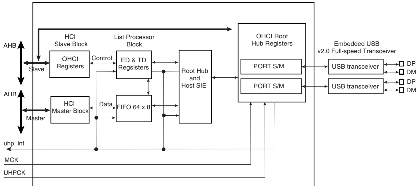
Figure 36-1. Block Diagram
