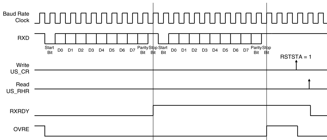
Figure 32-21. Receiver Status
