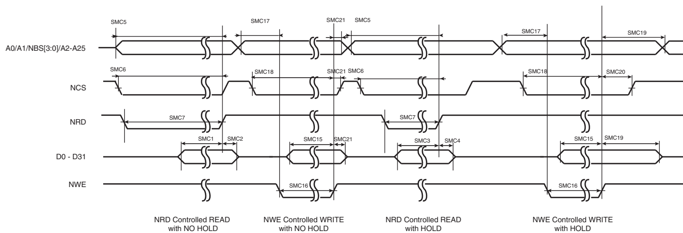
Figure 39-5. SMC timings - NRD controlled Read and NWE controlled Write
