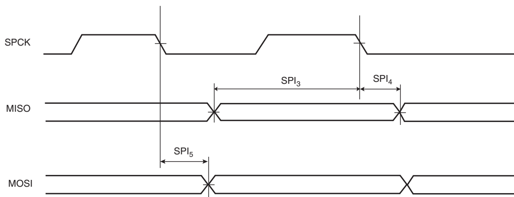
Figure 39-7. SPI Master Mode 0 and 3
