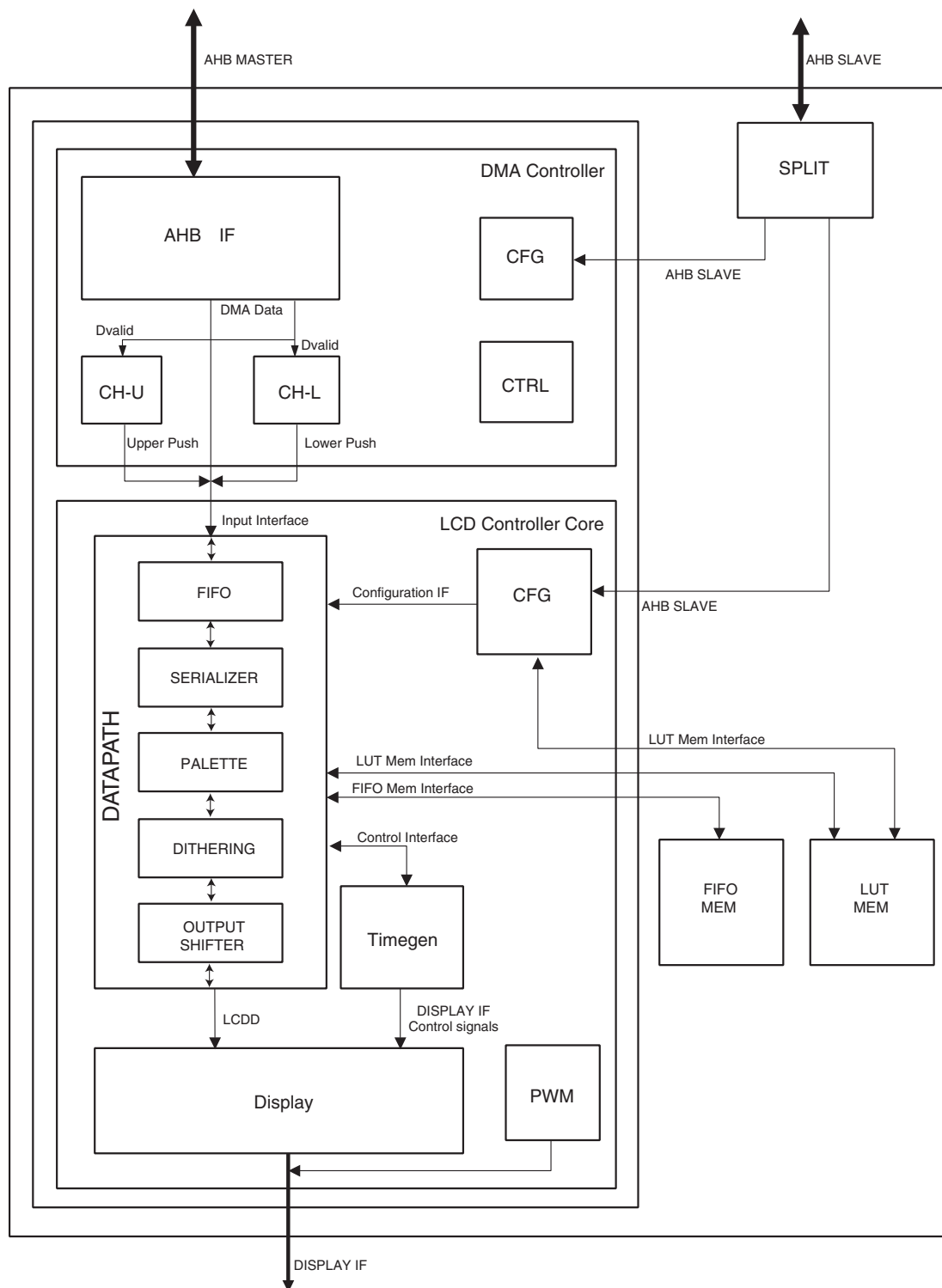
Figure 38-1. LCD Macrocell Block Diagram
