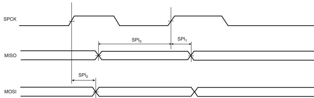
Figure 39-6. SPI Master Mode 1 and 2
