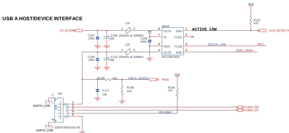
Figure 3-24. USB Port (A)
