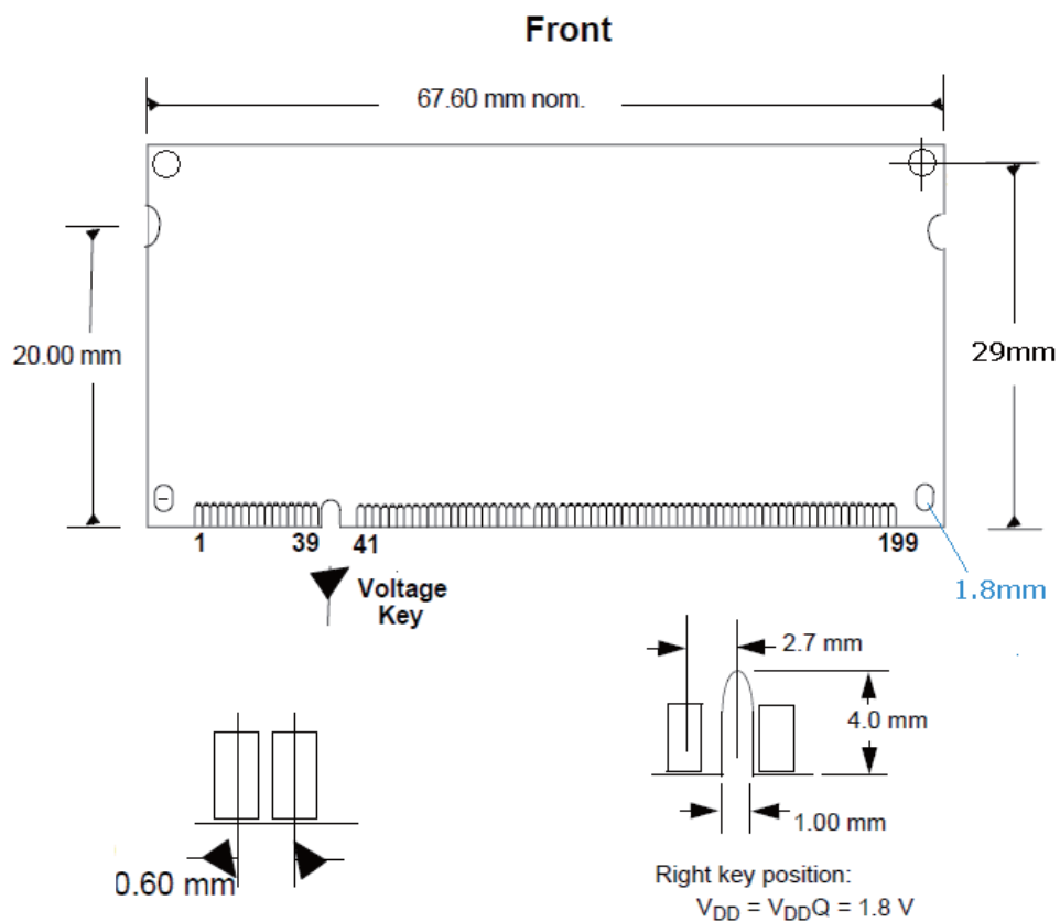
Figure 3-11. CM Board Dimensions
