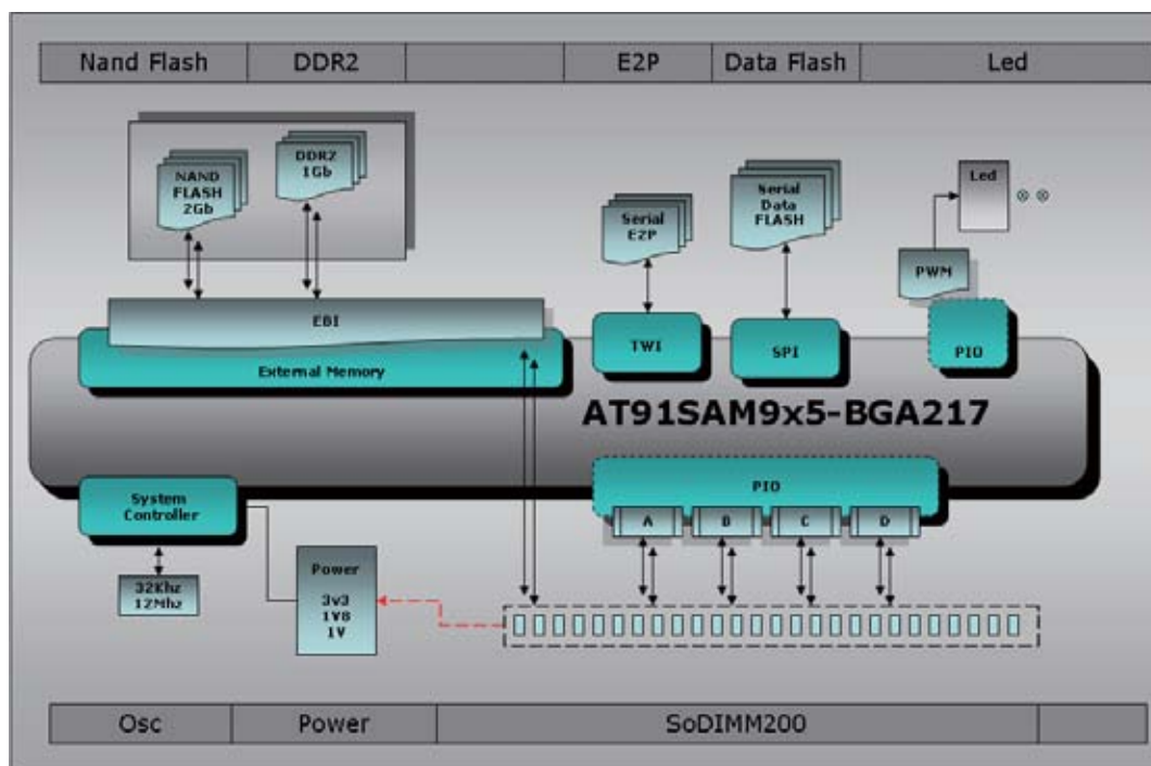
Figure 3-1. Board Architecture
