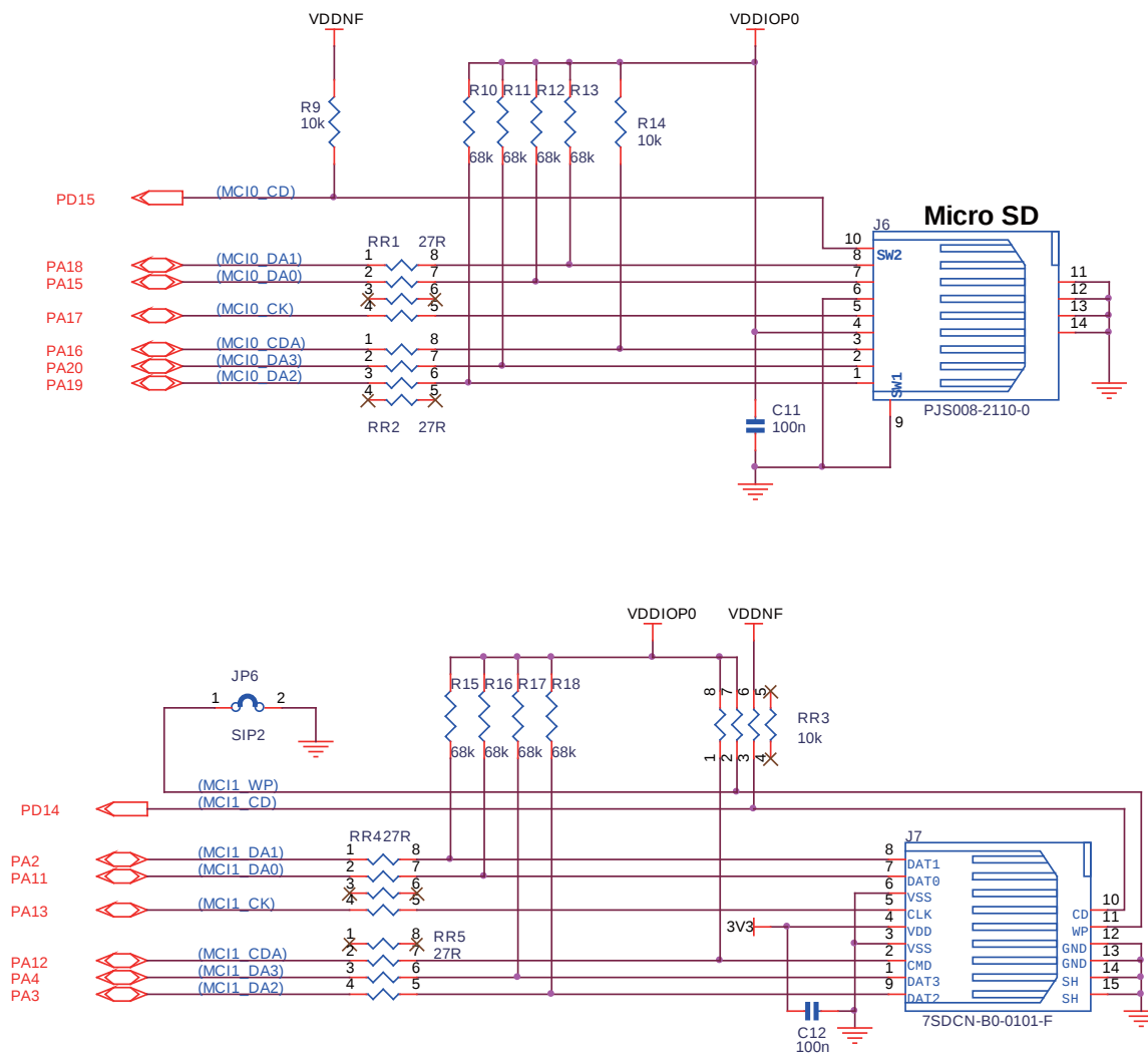
Figure 3-32. SD/MMC Interface
