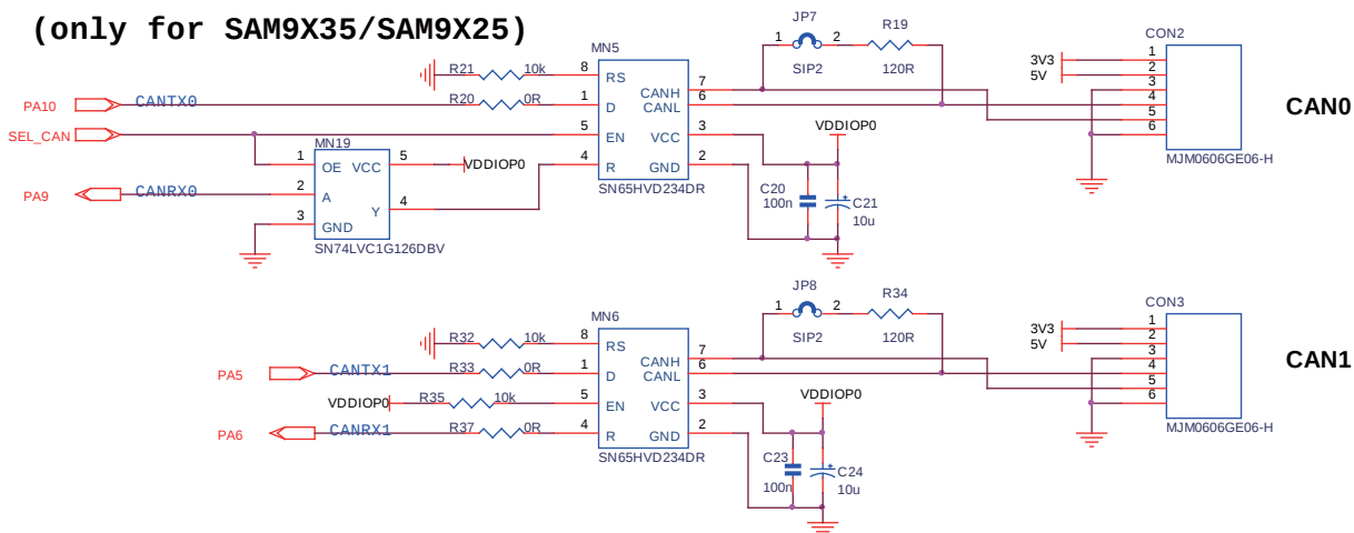
Figure 3-30. CAN on EK
