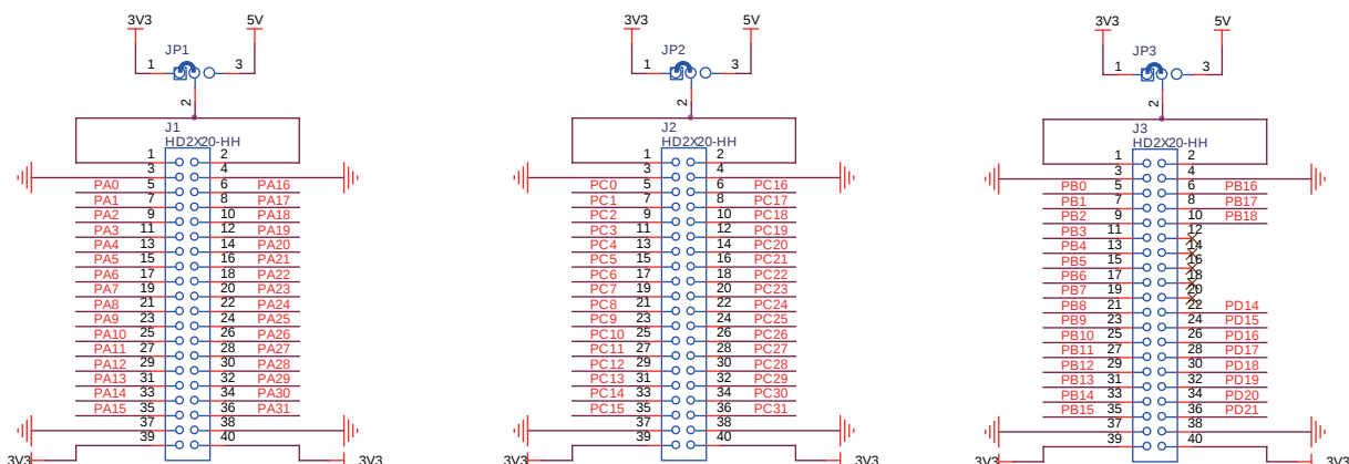
Figure 3-34. I/O Expansion
