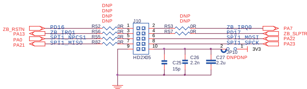
Figure 3-33. ZigBee Interface
