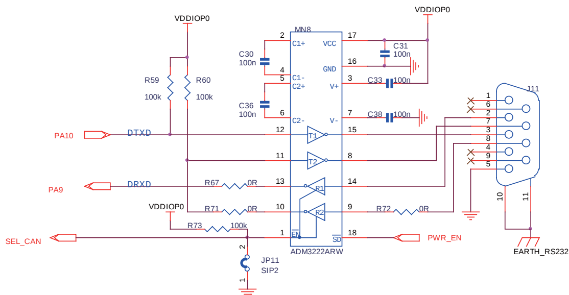
Figure 3-22. DBGU Com Port
