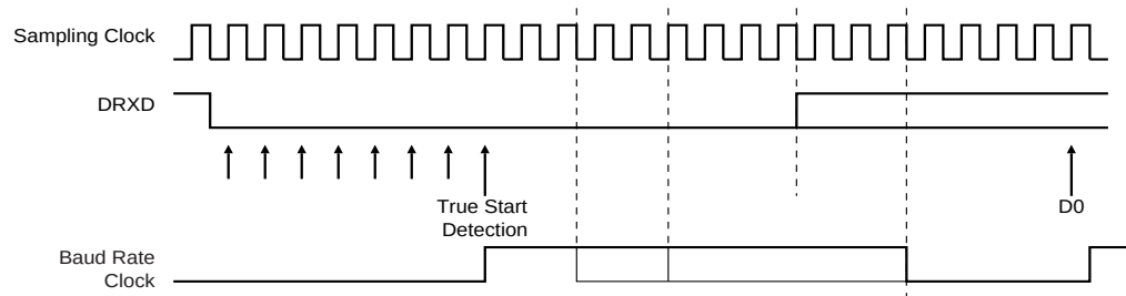
Figure 30-3. Start Bit Detection
