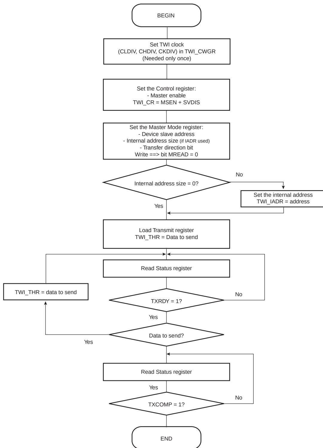
Figure 32-16. TWI Write Operation with Multiple Data Bytes with or without Internal Address
