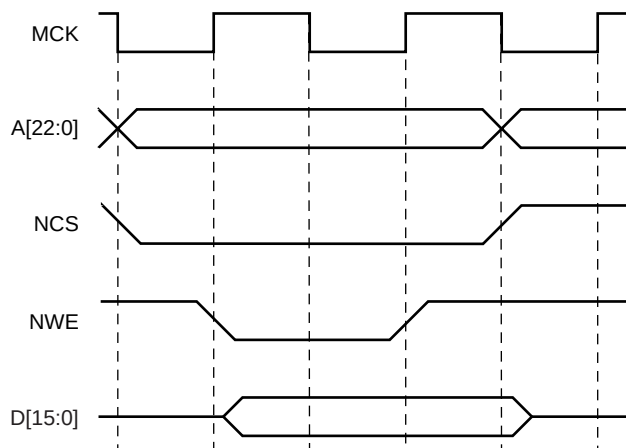
Figure 22-10. Write Access with 1 Wait State
