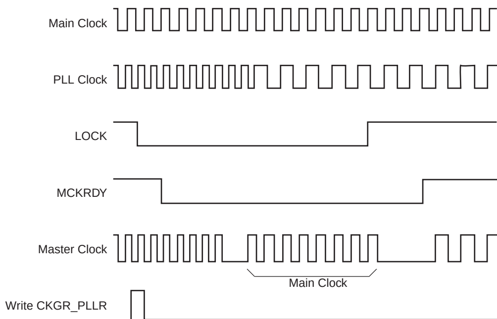
Figure 29-5. Change PLL Programming
