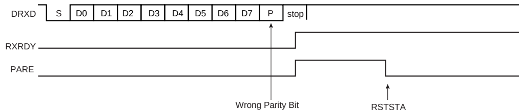
Figure 30-7. Parity Error
