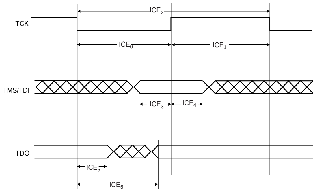
Figure 40-11. ICE Interface Signals
