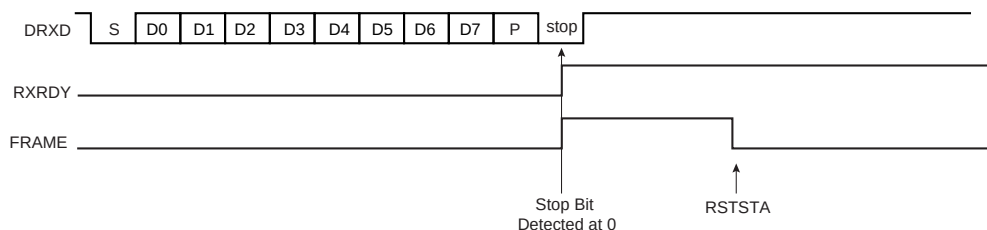
Figure 30-8. Receiver Framing Error
