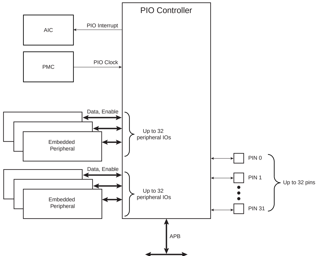
Figure 34-1. Block Diagram
