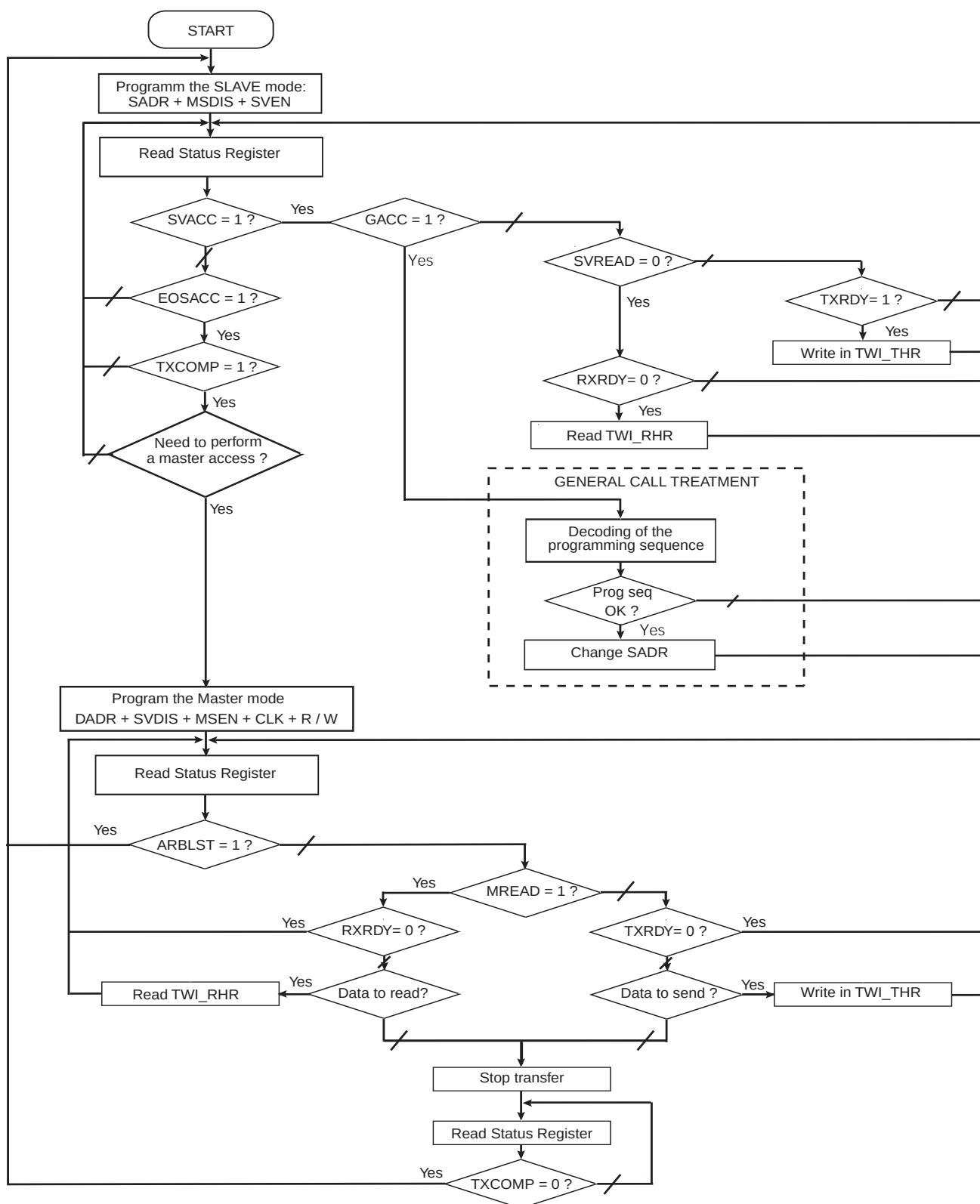
Figure 32-22. Multi-master Flowchart
