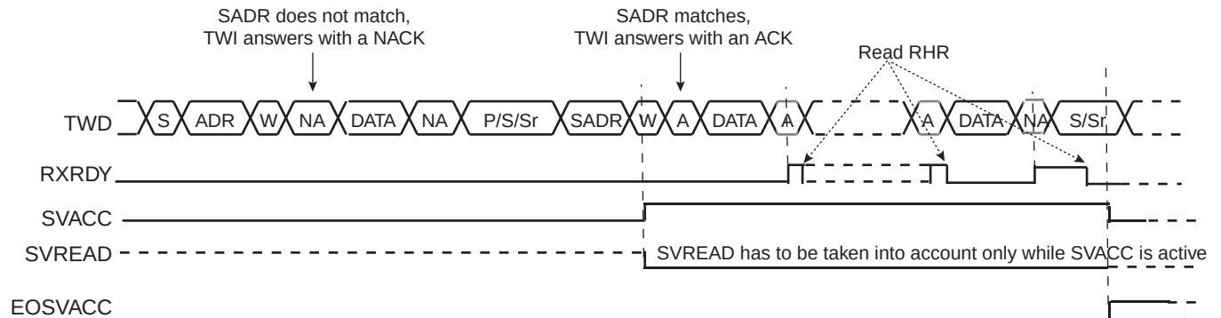
Figure 32-25. Write Access Ordered by a Master
