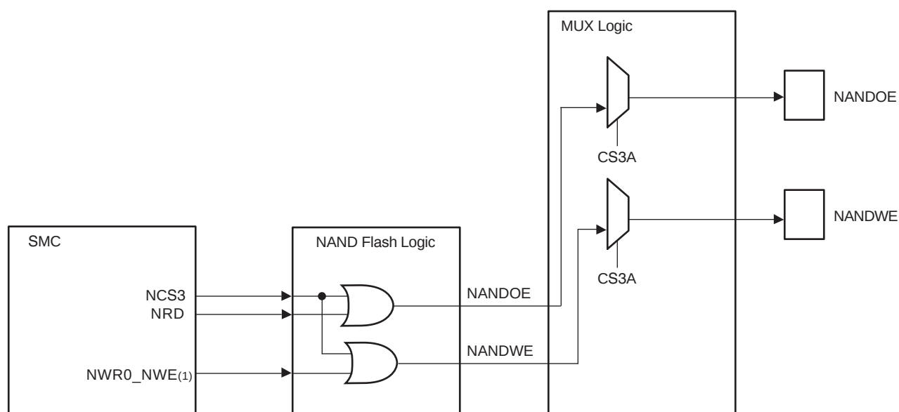
Figure 21-6. NAND Flash Signal Multiplexing on EBI Pins
