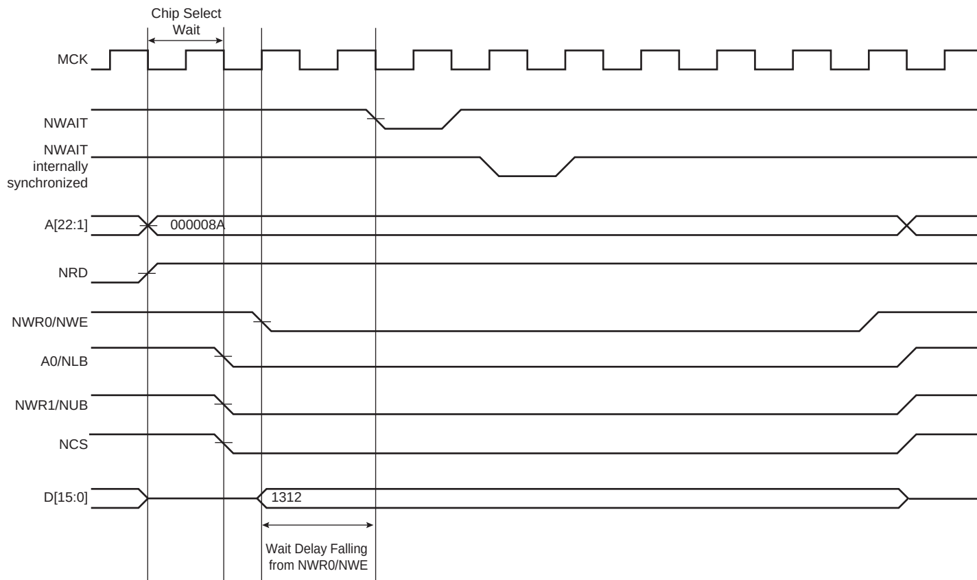
Figure 22-34. Write Access using NWAIT in Byte Select Type Access (1)
