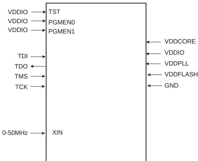
Figure 20-4. Serial Programming
