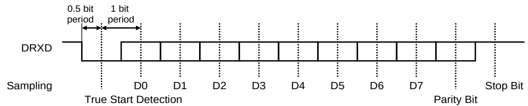
Figure 30-4. Character Reception
