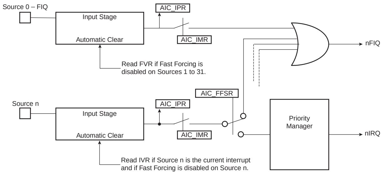
Figure 27-10. Fast Forcing
