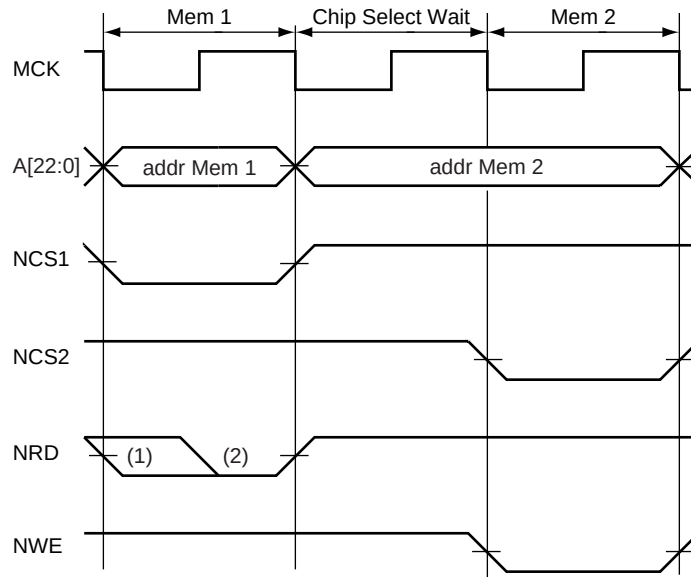
Figure 22-17. Chip Select Wait State
