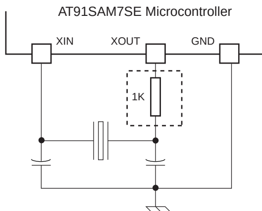
Figure 28-2. Typical Crystal Connection
