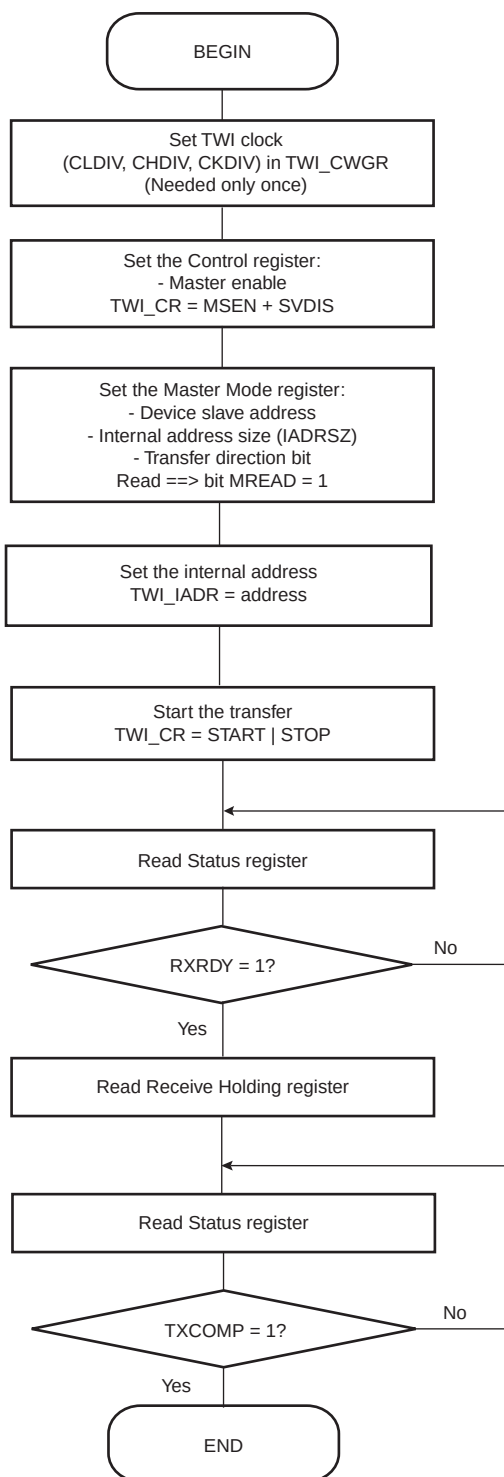
Figure 32-18. TWI Read Operation with Single Data Byte and Internal Address
