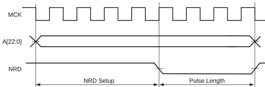
Figure 22-20. Read Access with Setup
