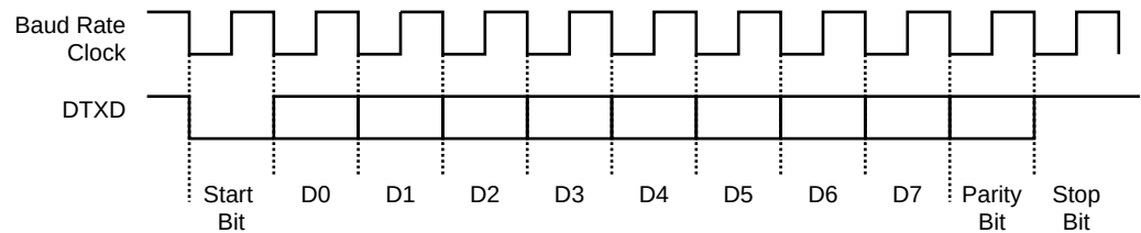
Figure 30-9. Character Transmission
