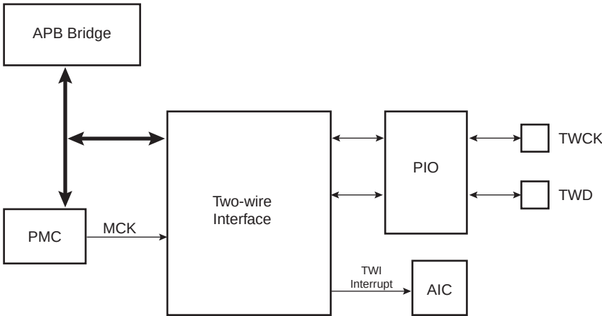
Figure 32-1. Block Diagram
