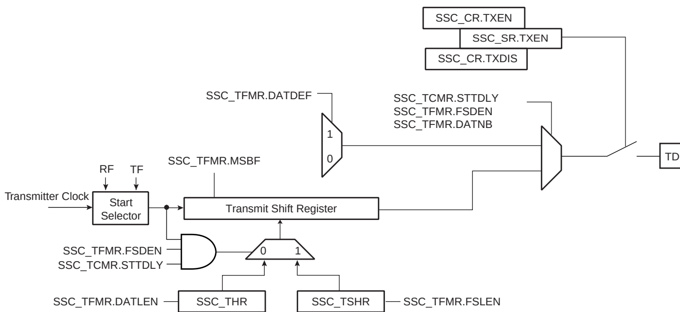
Figure 35-8. Transmitter Block Diagram
