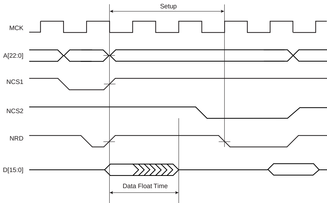
Figure 22-24. First Access with Data Float Wait States (TDF = 2) and Second Access with Setup (NRDSETUP = 1)
