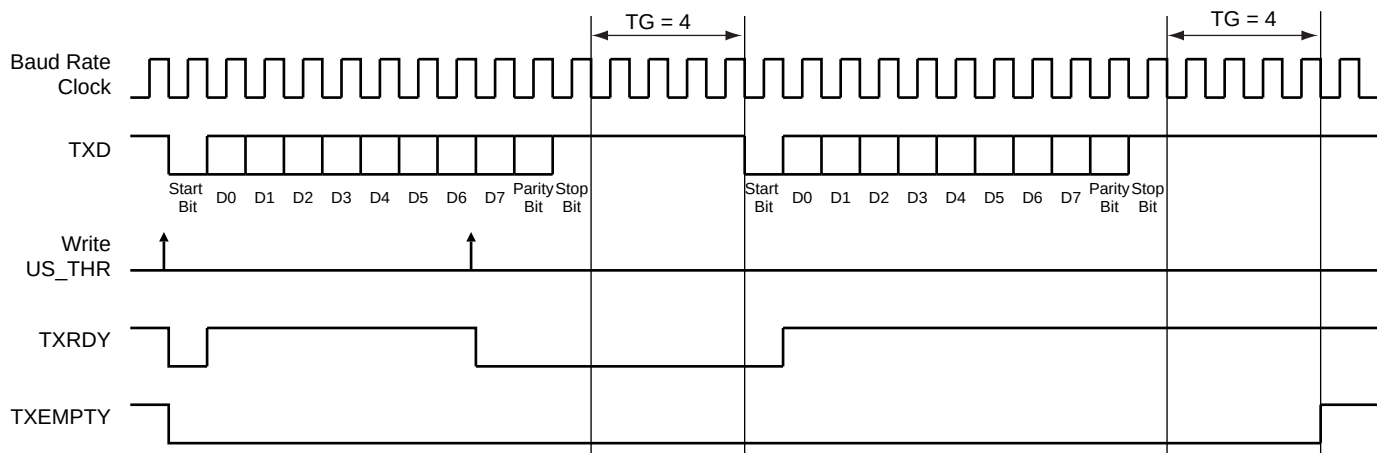
Figure 33-13. Timeguard Operations
