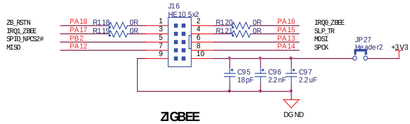
Figure 4-23. ZigBEE Interface
