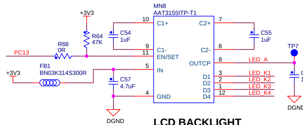
LCD BACKLIGHT
