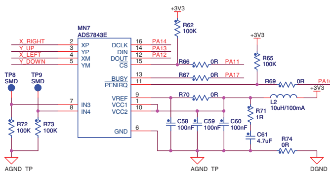
Figure 4-10. Touch Panel Control
